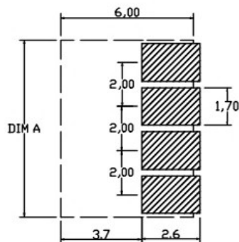
RECOMMENDED PCB LAYOUT TOP VIEW(.XX±0.05)
