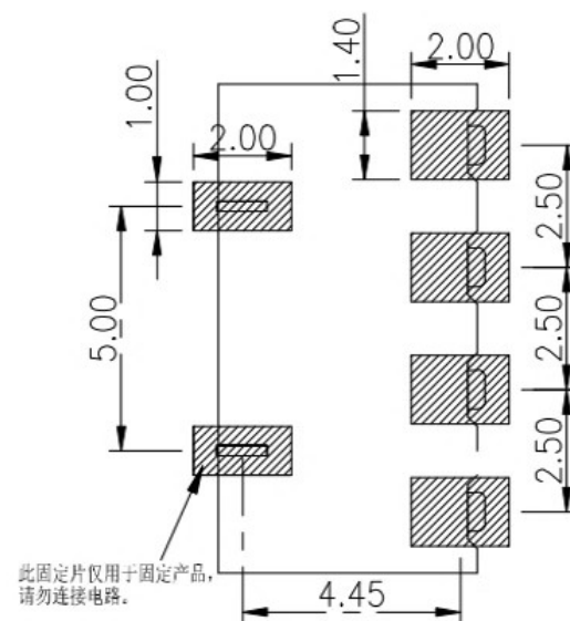
RECOMMENDED PCB LAYOUT TOP VIEW (.XX±0.05)
