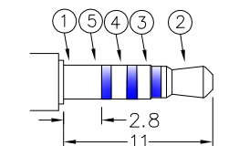
Ø2.5 MATE PLUG
