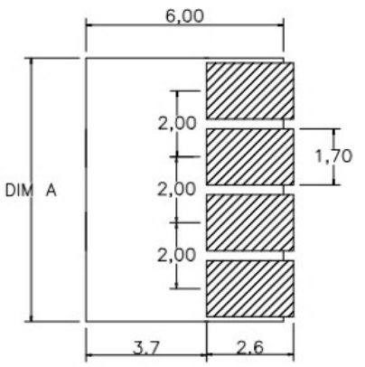
RECOMMENDED PCB LAYOUT TOP VIEW(.XX±0.05)
