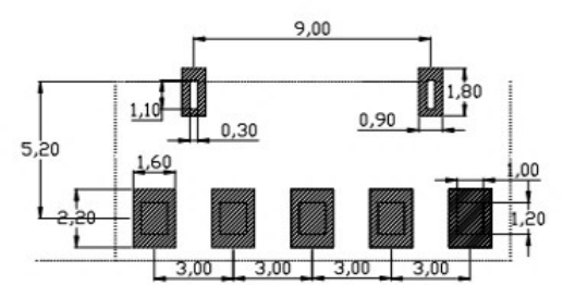
RECOMMENDED PCB LAYOUT TOP VIEW(.XX±0.05)
