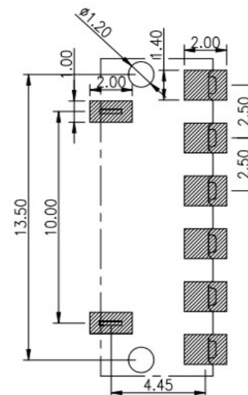
RECOMMENDED PCB LAYOUT TOP VIEW (.XX±0.05)
