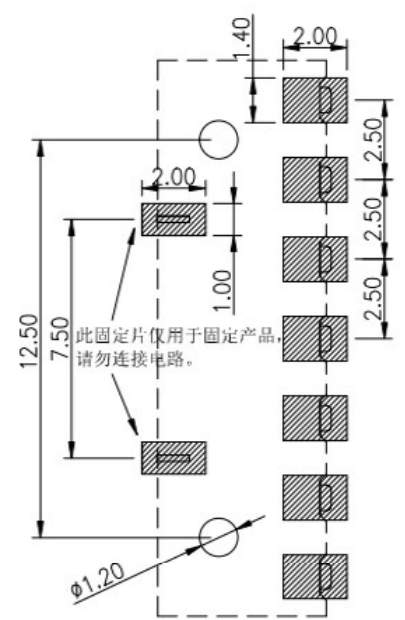
RECOMMENDED PCB LAYOUT TOP VIEW (. XX±0. 05)
