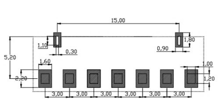
RECOMMENDED PCB LAYOUT TOP VIEW (XX±0.05)
