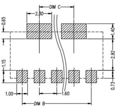
RECOMMENDED PCB LAYOUT TOL:(±0.05)
