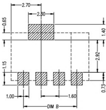
RECOMMENDED PCB LAYOUT TOL:(±0.05)
