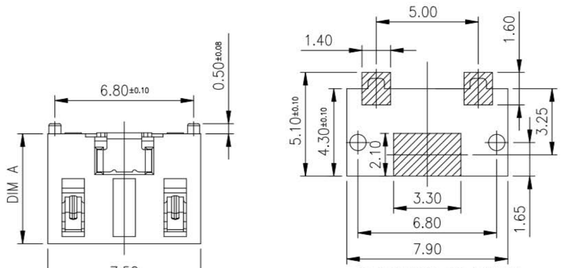
RECOMMENDED PCB LAYOUT TOP VIEW (.XX±0.05)
