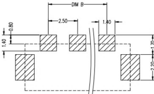
RECOMMENDED PCB LAYOUT TOL:(±0.05)
