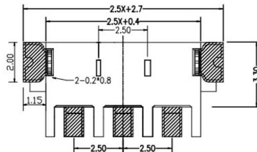
PCB LAYOUT (3pin)
