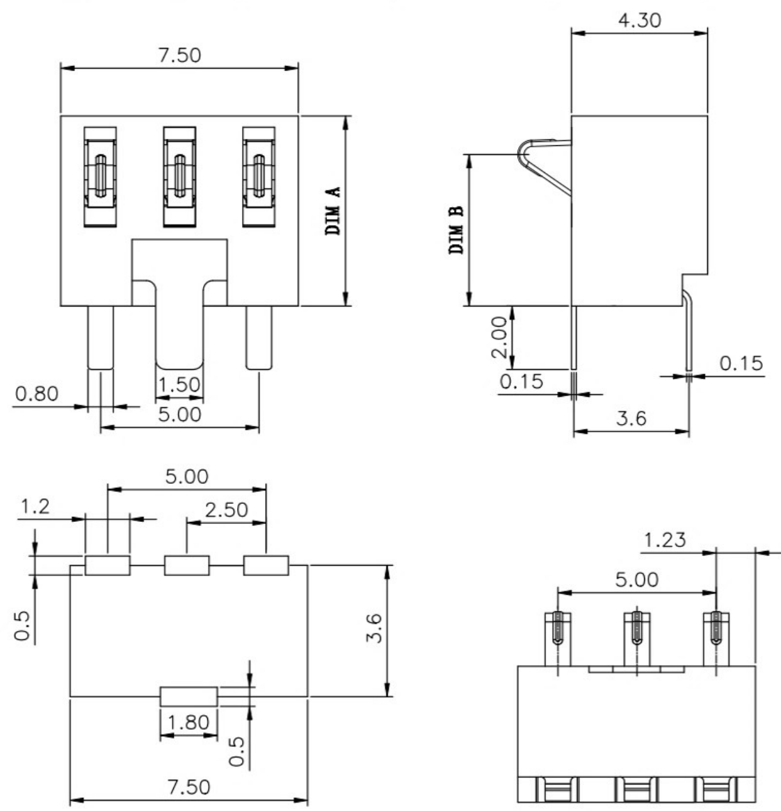
RECOMMENDED PCB LAYOUT TOP VIEW(. XX±0.05)
