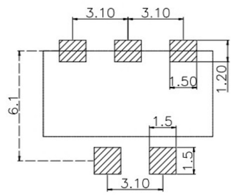
PCB Layout
