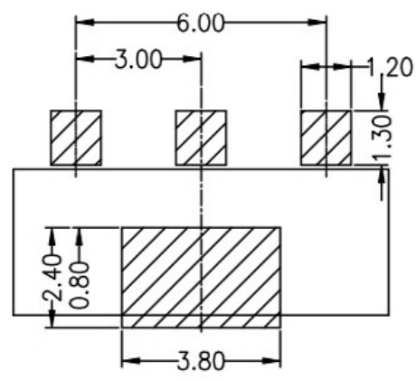
RECOMMENDED PCB LAYOUT TOL:(±0.05)
