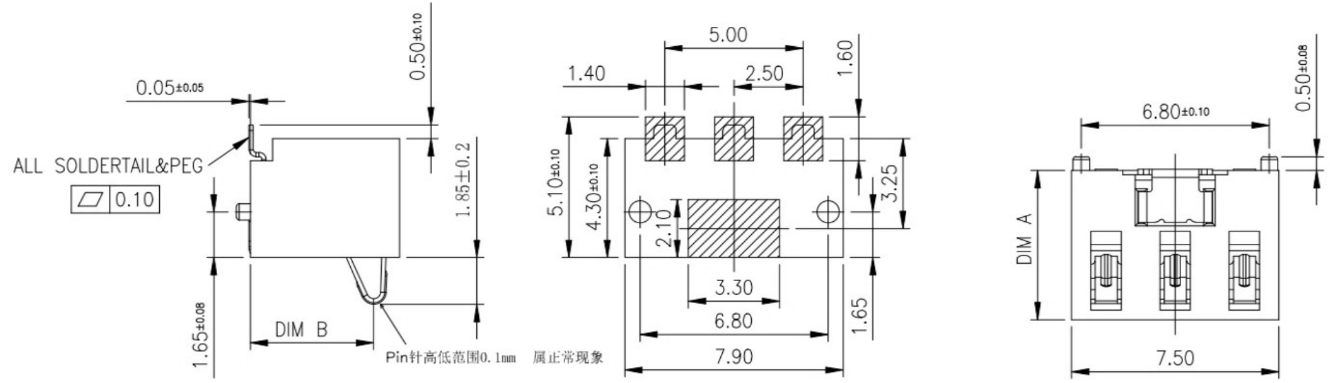
RECOMMENDED PCB LAYOUT TOP VIEW (.XX±0.05)
