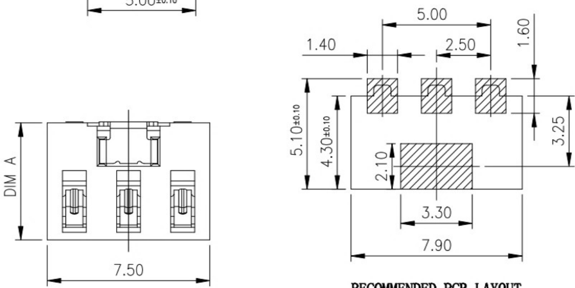
RECOMMENDED PCB LAYOUT TOP VIEW(. XX±0.05)
