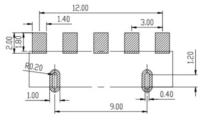
RECOMMENDED PCB LAYOUT TOL:( \pm 0.05 )
