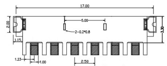
PCB LAYOUT(6pin)
