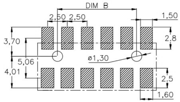
RECOMMENDED PCB LAYOUT TOP VIEW (.XX±0.05)
