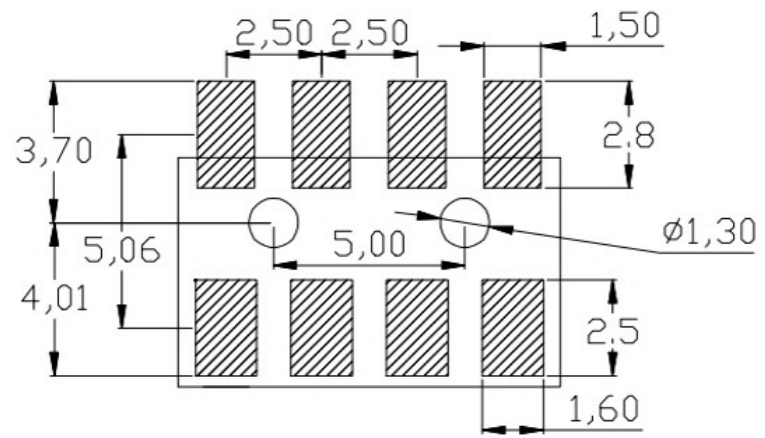
RECOMMENDED PCB LAYOUT TOP VIEW (. XX \pm 0.05)
