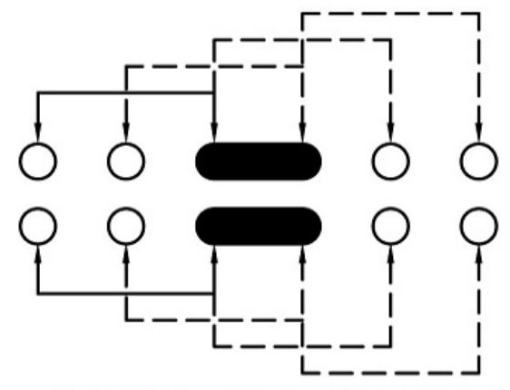
SCHEMATIC (NON-SHORTING)
