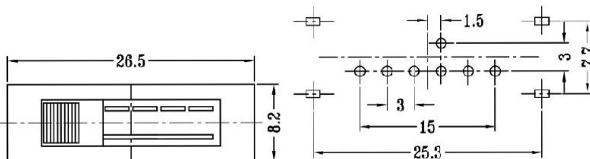
P.C.B LAYOUT BOTTOM VIEW
