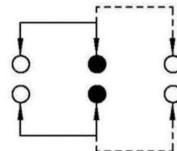
SCHEMATIC (NON-SHORTING)
