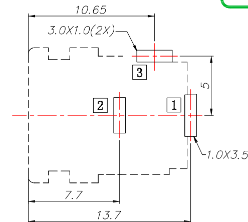
RECOMENDED P.C.B LAYOUT (BOTTOM VIEW)
