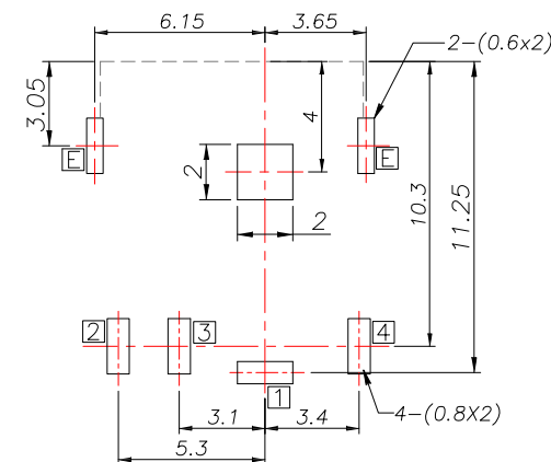
PCB LAYOUT MOUNTING PATTERN (BOTTOM VIEW)
