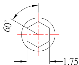
SHAFT HOLE SHAPE AND DIMENSION
