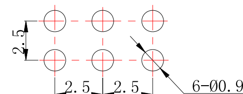
P.C.B LAYOUT MOUNTING PATTERN
