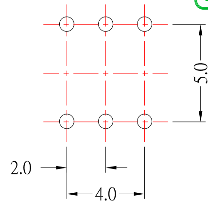
P.C.B MOUNTING PATTERN BOTTOM VIEW
