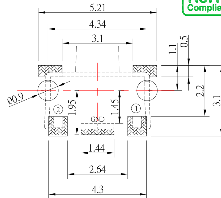
P.C.B. LAYOUT MOUNTING PATTERN
