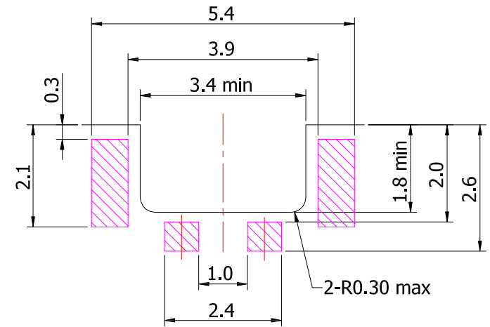
PCB LAYOUT
