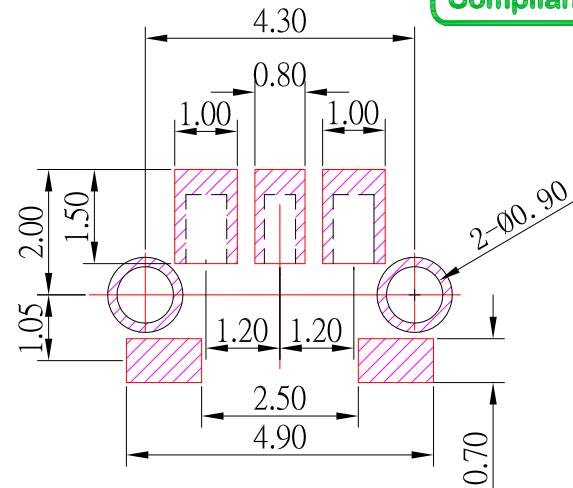
PCB LAYOUT
