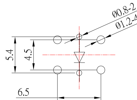
MOUNTING PATTERN
