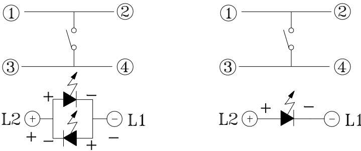
CIRCUIT DIAGRAM
