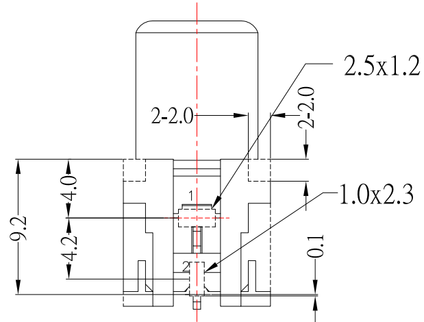
PCB HOLES DIAGRAM BOTTOM VIEW
