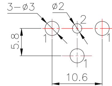
PCB HOLES DIAGRAM TOP VIEW
