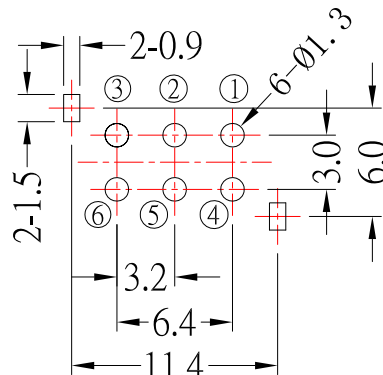
P.C.B LAYOUT MOUNTING PATTERN BOTTOM VIEW
