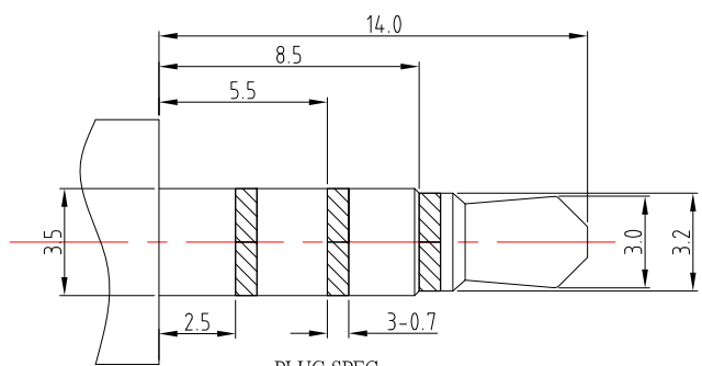
PLUG SPEC
