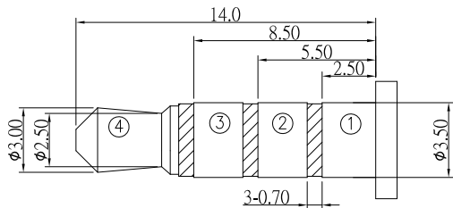
(φ3.50mm 4 POLE PLUG DETAIL DRAWING)
