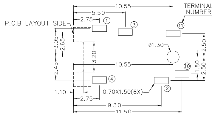
RECOMMENDED (BOTTOM VIEW)
