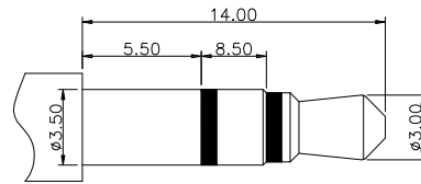
Ø3.50mm 3 POLE PLUG
