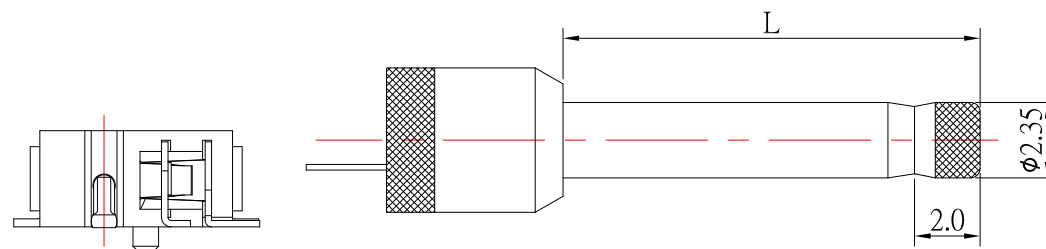
RECOMMENDED PLUG
