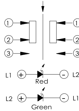
CIRCUIT
