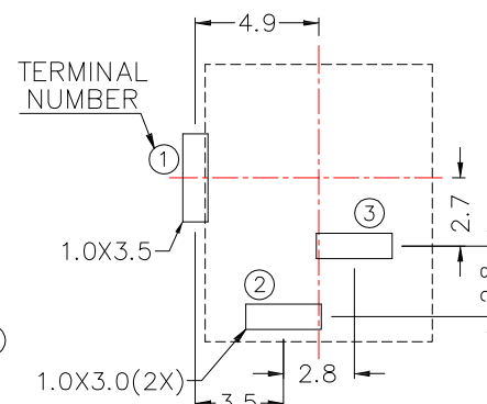
P.C.B LAYOUT MOUNTING PATTERN (TOP VIEW)
