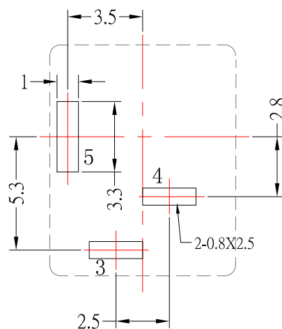
P.C.B LAYOUT MOUNTING PATTERN (TOP VIEW)
