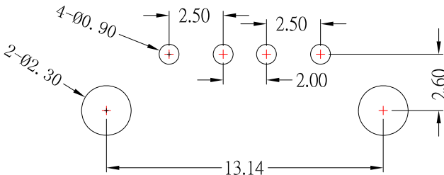
P.C.B LAYOUT MOUNTING PATTERN
