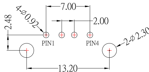
P.C.B LAYOUT MOUNTING PATTERN
