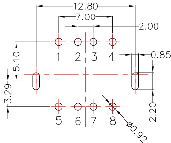
P.C.B LAYOUT MOUNTING PATTERN
