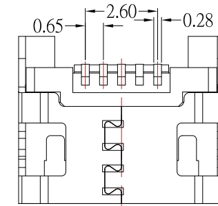
P.C.B LAYOUT MOUNTING PATTERN
