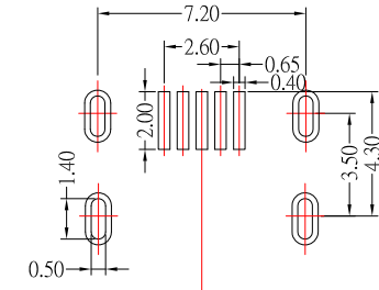
P.C.B LAYOUT MOUNTING PATTERN
